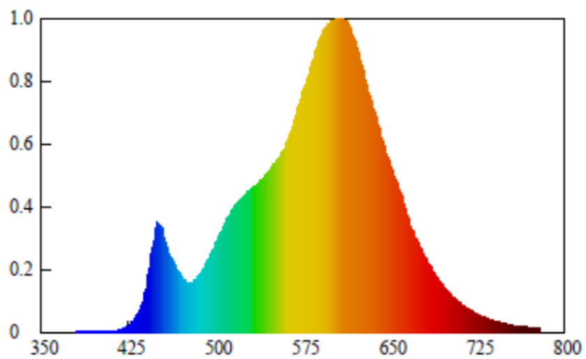
Spectral Distribution
