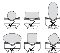
The universal bracket fits most tube shapes.
