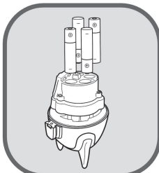
4. Use good quality Alkaline or NiMH rechargeable AA batteries making sure that the flat end of each battery (negative) touches the contact spring. Do not use low power zinc batteries.
