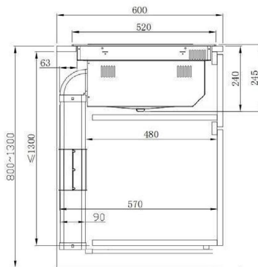
Utsugningsversion
